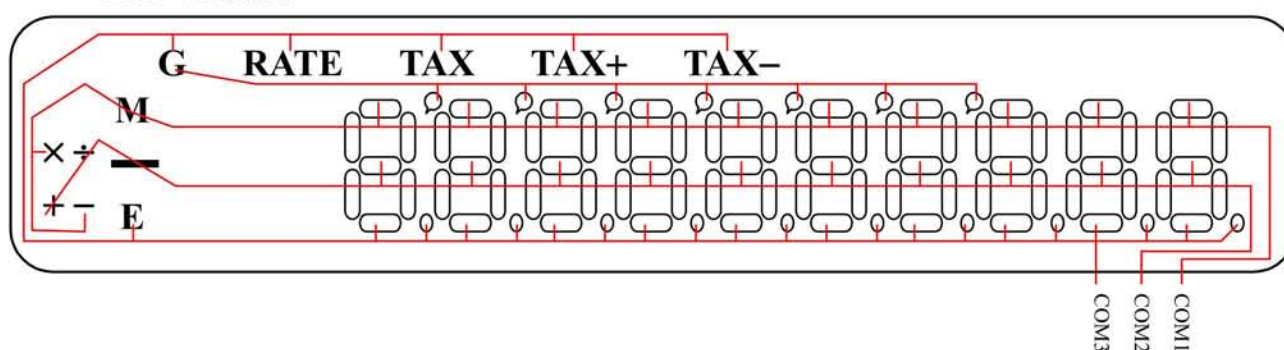
LCD Common
