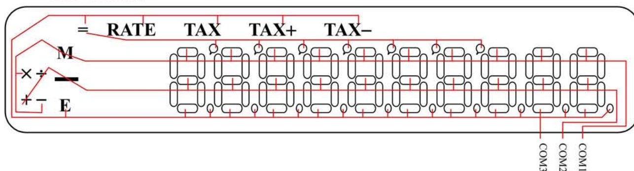
LCD Common
