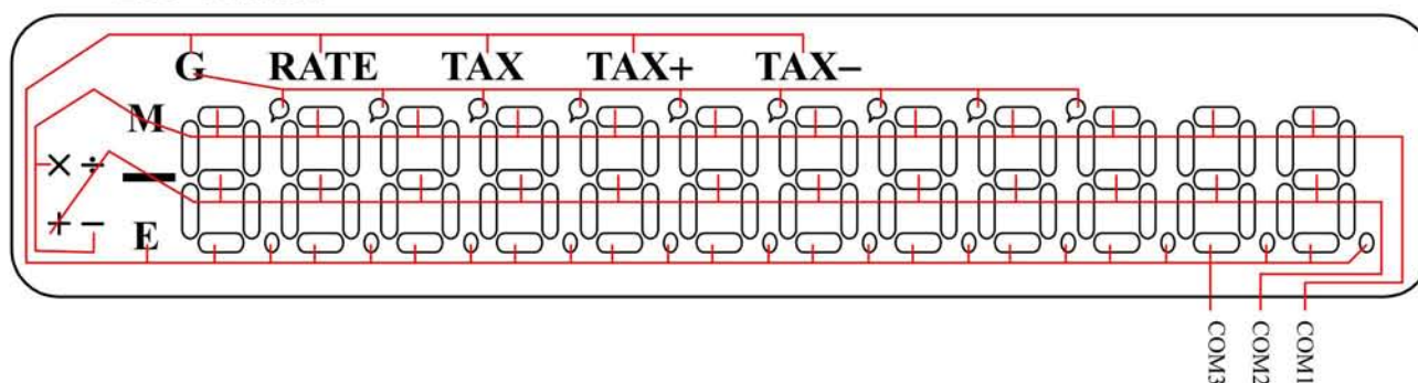
LCD Common
